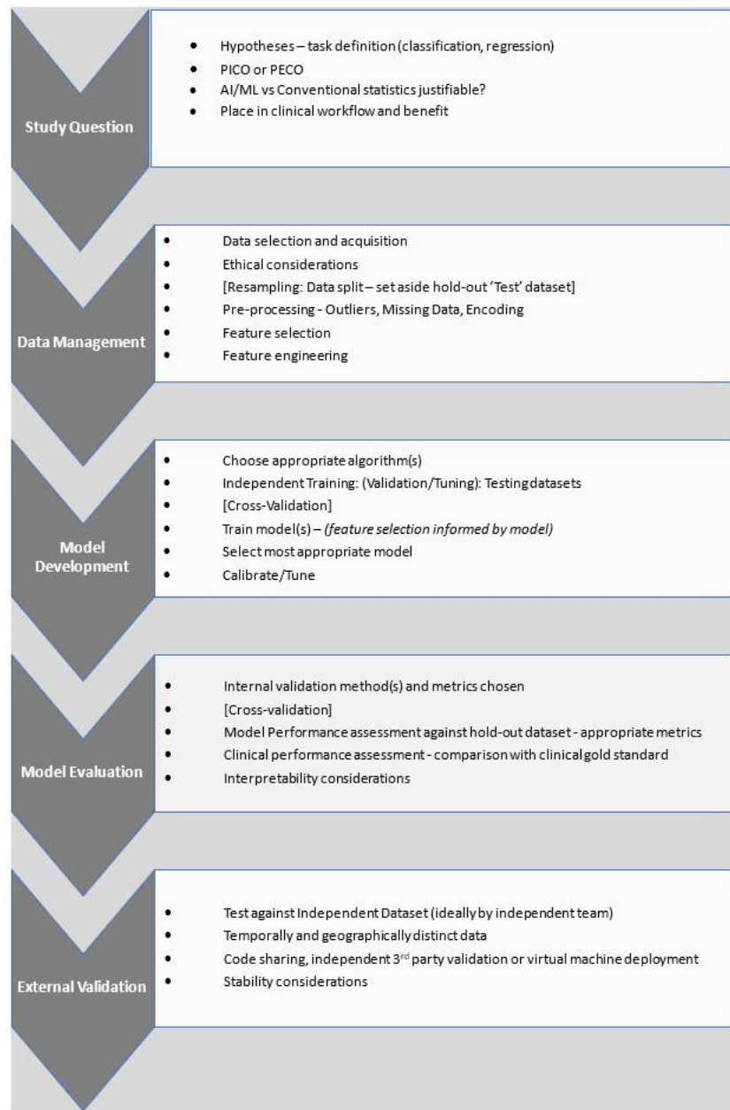
Figure 2 Steps in artificial intelligence (AI) model development. Square brackets denote steps which are sometimes described during data management, model development or evaluation. Feedback and iterations of preceding steps are expected. ML, machine learning. PICO/PECO - Population/ Intervention (Exposure)/Comparison/Outcome
